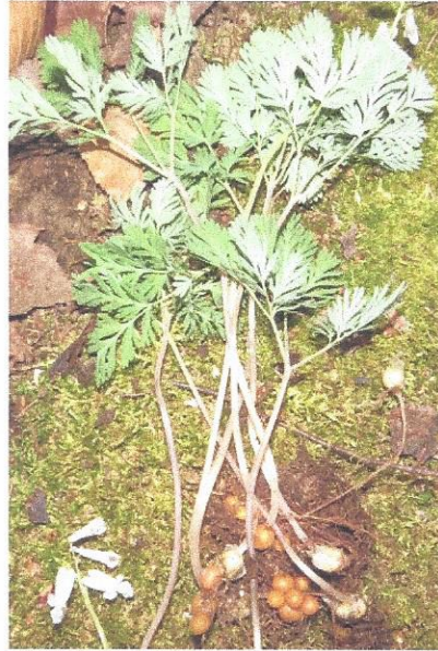
Squirrel corn and its root tubers
